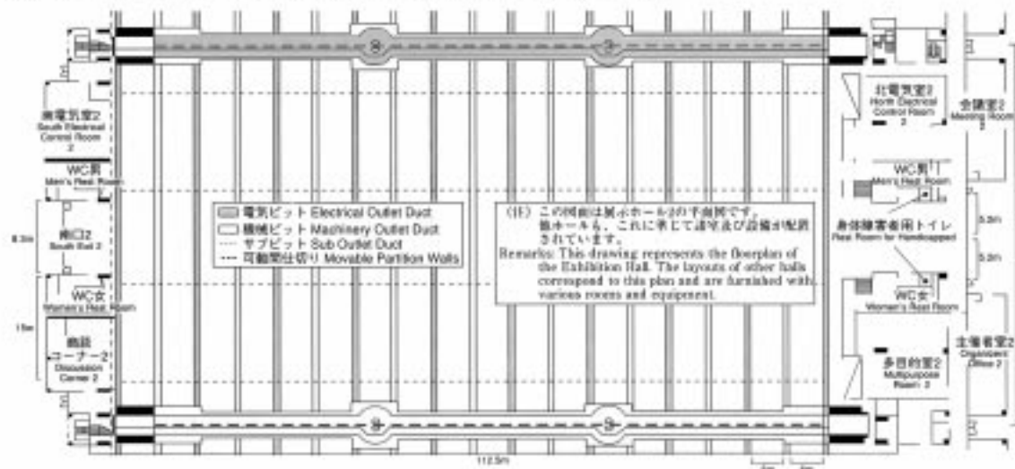
展示ホール1階平面図 Layout of Exhibition Hall 2, 1st Floor
